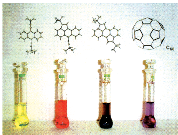
Figure 1. Dilute toluene solutions of compounds 2a , 2b , and 2c illustrating the remarkable changes in UV–vis absorption spectra as a function of mono- and bis-cyclopenteneation. A dilute solution of C 60 is also shown for comparison.
