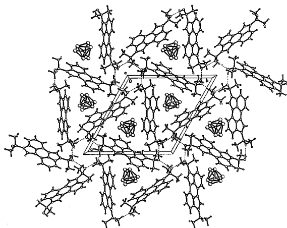
Figure 5. Crystal packing diagram of 2c down the c -axis direction illustrating hydrogen bonding in an hexagonal array as shown with dotted lines. Disordered dichloromethane solvent molecules sit in a 3-fold axis of symmetry.
